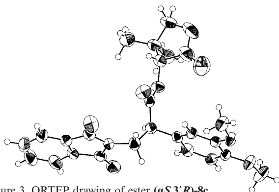
Figure 3. ORTEP drawing of ester ( \alpha,S,3'R )- 8c
