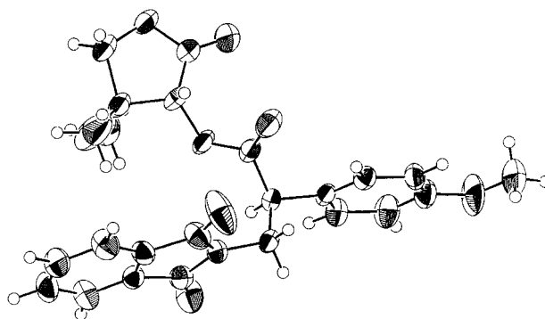
Figure 1. ORTEP drawing of ester ( \alpha S, 3'R )- 8a
