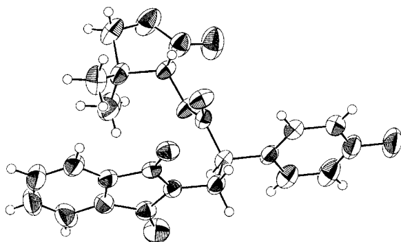
Figure 2. ORTEP drawing of ester ( \alpha,S,3'R )- 8b
