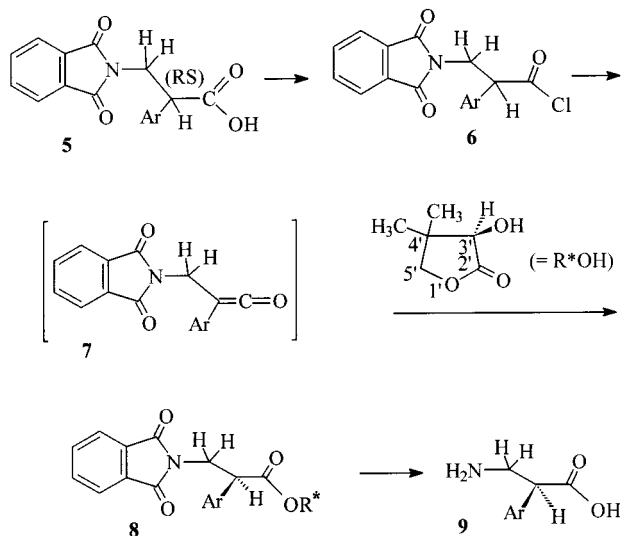
Scheme 3. Stereoselective synthesis of 9a–d
